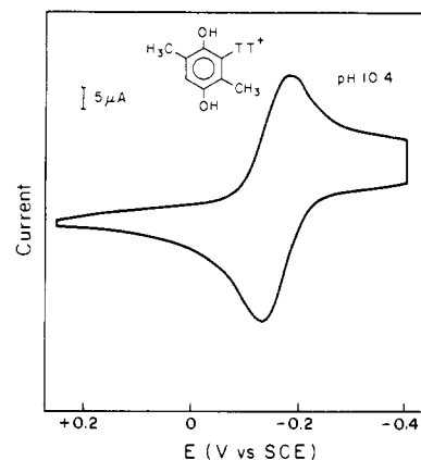
Figure 1. Cyclic voltammogram of 6 , pH 10.4, \mu = 0.5 , T = 23^\circ\text{C} , scan rate = 100 mV/s.
