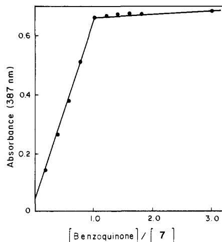
Figure 3. Mole-ratio plot for the oxidation of 7 by p -benzoquinone at pH 6.0.
