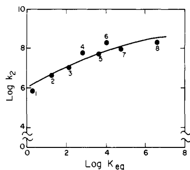
Figure 6. Correlation of \log k_2 with \log K_{eq} . The curve is calculated from eq 18 and 19. The numbers refer to reactions described in Table III.
