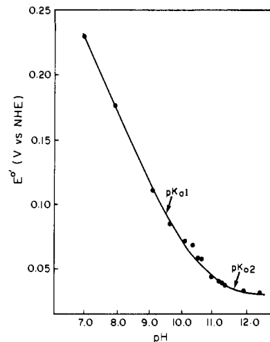
Figure 2. Dependence of observed redox potential of 7 upon pH; \mu = 0.5 , T = 23^\circ\text{C} .
