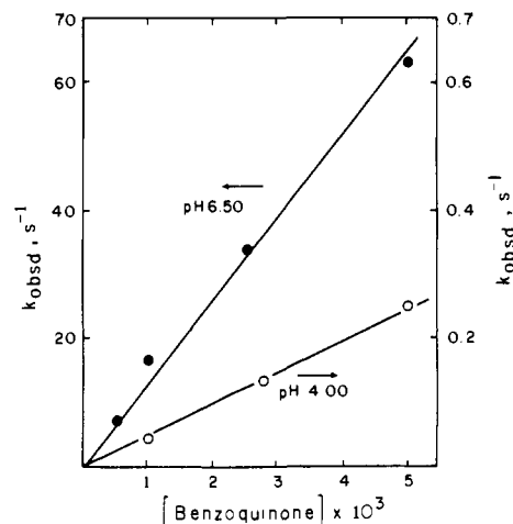
Figure 4. Dependence of k_{\text{obsd}} upon oxidant concentration for the oxidation of 7 by p -benzoquinone at pH 4.0 ( r = 0.9991 ) and 6:5 ( r = 0.9990 ).
