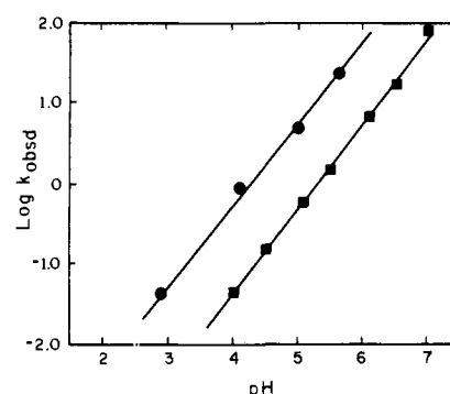
Figure 5. Dependence of k_{\text{obsd}} upon pH for the oxidation of 7 (■, slope = 1.06 \pm 0.06 , r = 0.9921 ) and 8 (●, slope = 1.02 \pm 0.02 , r = 0.9997 ) by p -benzoquinone ( 1.0 \times 10^{-3} M).
